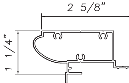
Ames Brickmould M2154
