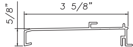
1 7/16 inch Brickmold Sill Nose M17610
