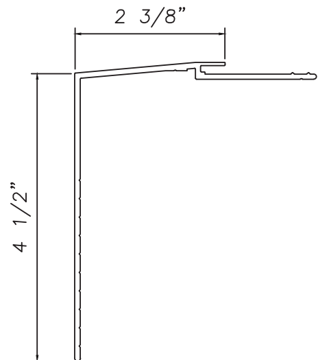
Sill Panning M19165
