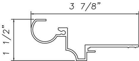
Breslyn House Panning M21397
