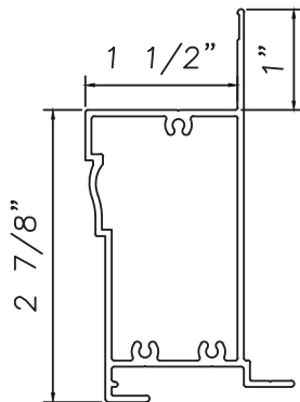
2 7/8 inch Brickmold M15494
