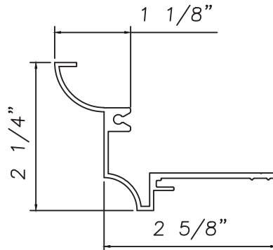
Breslyn House Panning 2 M21398
