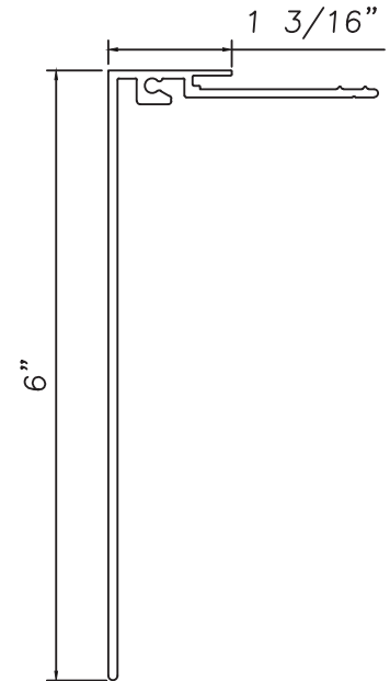
1"x6" Panning M19163
