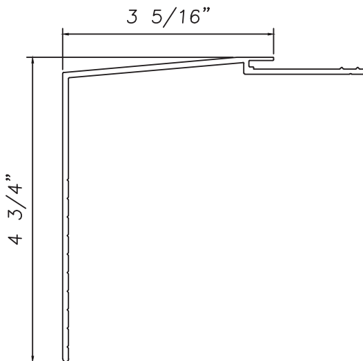
3" Sill Panning M19164
