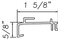
Brickmold Sill Nose M17609
