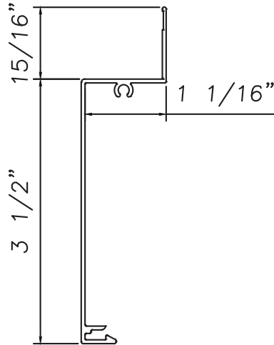
Molding Panning M16380
